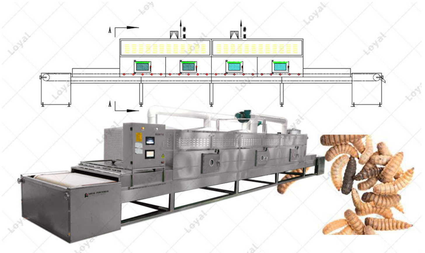
Detail of Industrial Conveyor Belt Type Microwave Oven For Black Soldier Fly Larvae Layout
