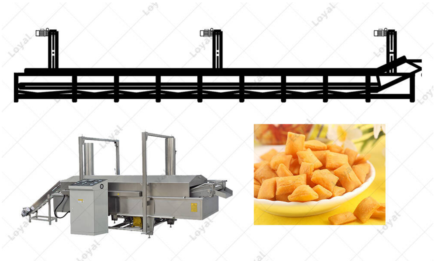
CAD Of Automatic Continuous Fryer Processing Line For Chin Chin Detailed Parameter of Industrial Continuous Frying Machine Commercial Automatic Chin Chin Fryer Machine
