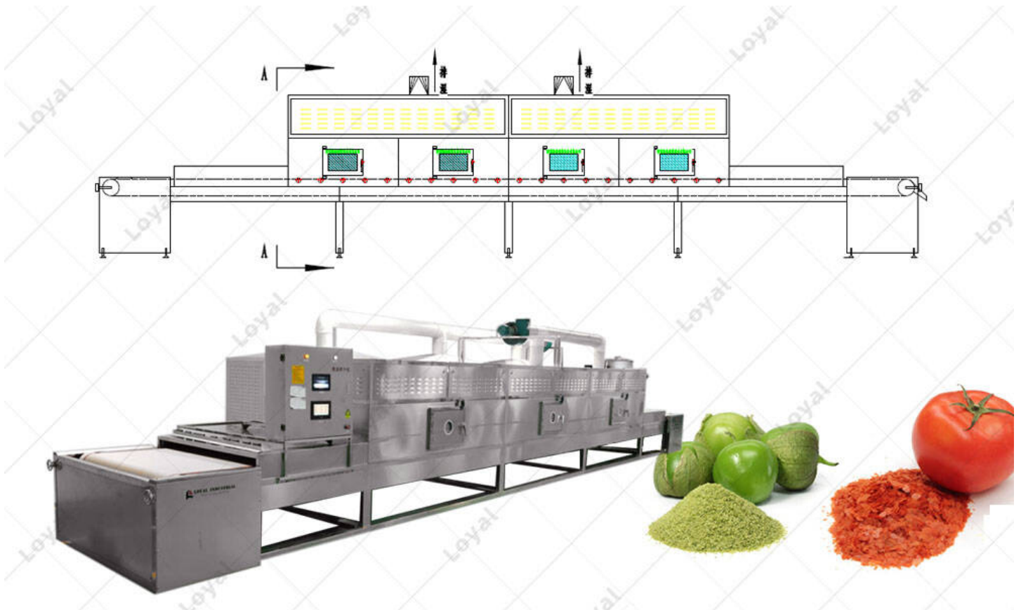
CAD of Continuous Dehydrated Vegetables Powder Microwave Sterilization Machine
