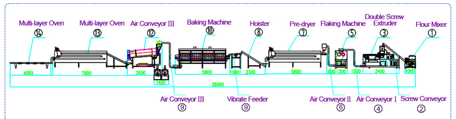
Flow Chart of Corn Flakes Production Line
