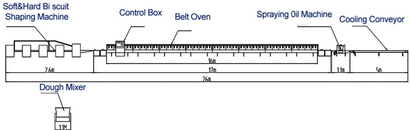
Flow Chart Of Automatic Biscuit Making Production Line
